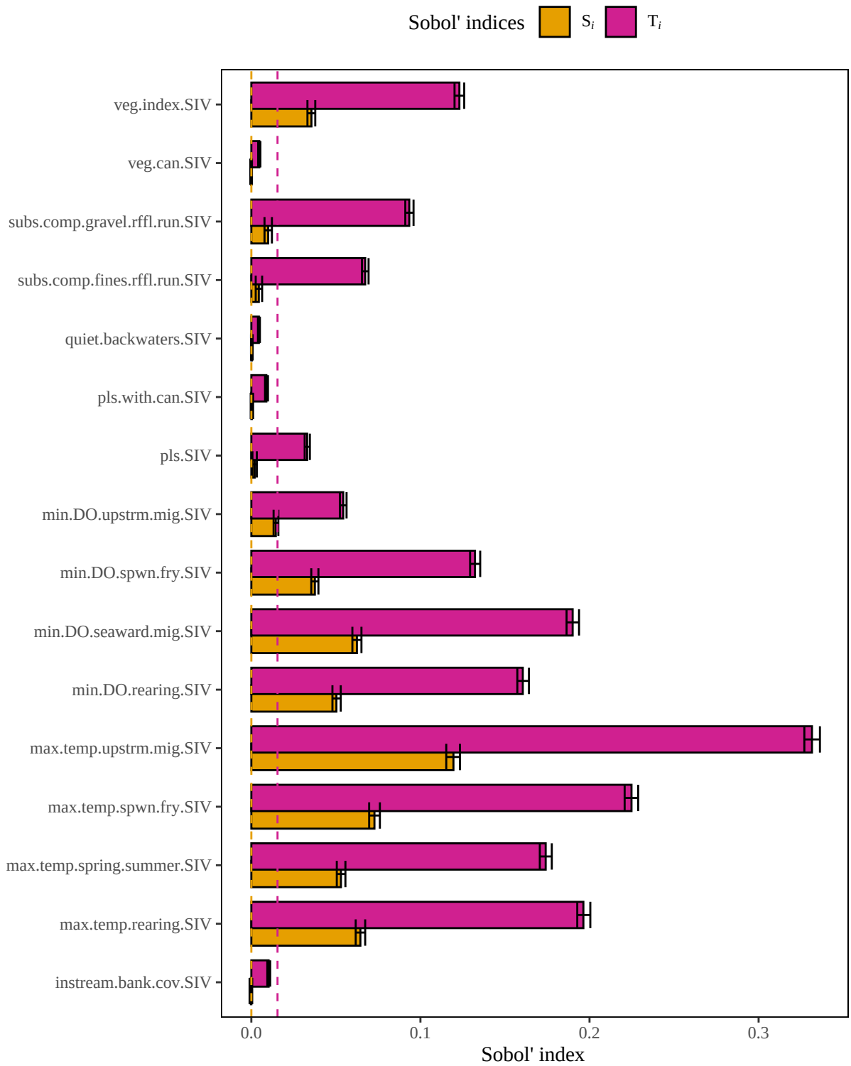
Figure 3. Results of a sensitivity analysis for the cohosalmonSpringSummerSeaMig model based on the original limiting factor model outlined in McMahon (1983). Dashed lines represent baseline numerical approximation error for S_i and T_i ( i.e. , dummy variables).
