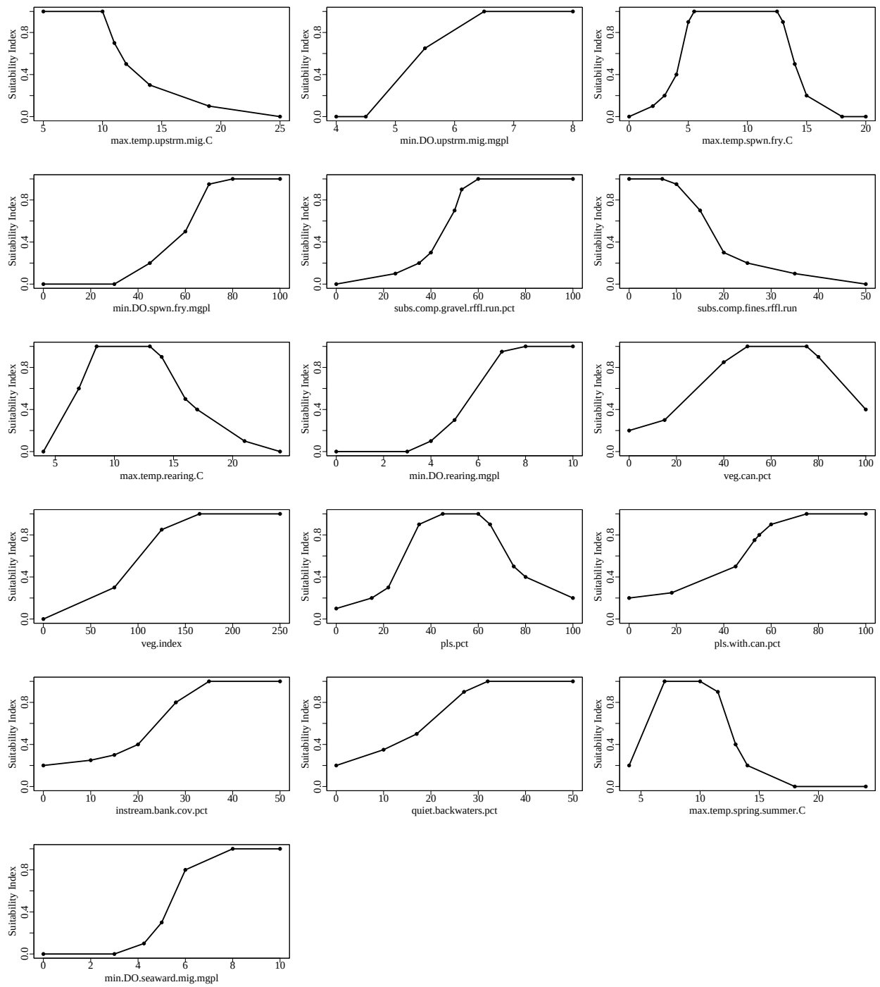
Figure 1. Suitability index graphs for variables included in the cohosalmonSpringSummerSeaMig model in ecorest.
